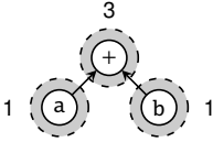
(c) Invalid cover due to incompatibilities between the selected patterns.
