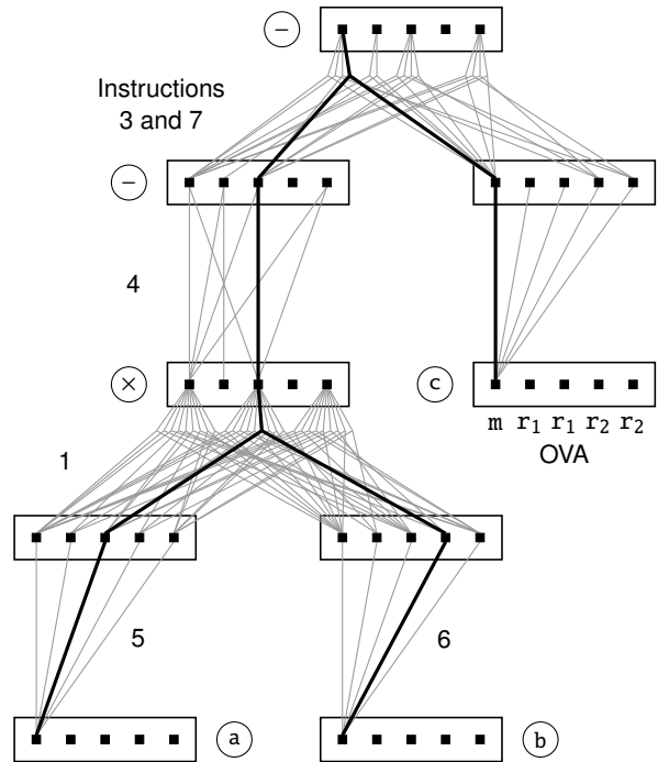
(c) Trellis diagram. Gray edges represent available paths, and black edges indicate the (selected) optimal path.
