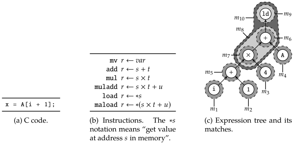
Figure B.1: Example demonstrating the pattern matching and selection problem for a function that loads a value from integer array A at offset i + 1 . It is assumed that i is stored in register, that A is stored in memory, and that an integer is four bytes. Exact covers are \{m_1, \dots, m_7, m_9\} , \{m_1, \dots, m_5, m_8, m_9\} , \{m_1, \dots, m_5, m_{10}\} , \{m_1, \dots, m_5, m_8, m_9\} (for brevity, non-exact covers are ignored). Variable assignments need not be explicitly represented as nodes since this information can be propagated from the root node after having found a cover.
