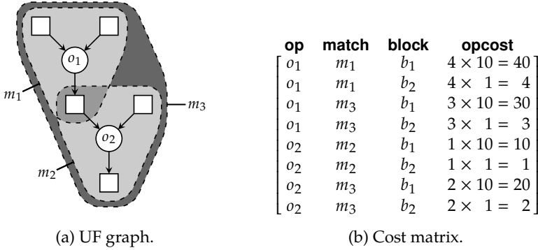
Figure 6.2: Example of match costs distributed over operations. It is assumed that matches m_1 , m_2 , and m_3 have costs 4, 1, and 5, respectively, and that they can be placed in one of two blocks, b_1 and b_2 , with execution frequencies 10 and 1, respectively. The cost of m_3 distributed over o_1 and o_2 is 3 and 2, respectively.
