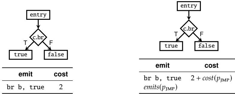
Figure 5.12: Example of creating a DTB pattern.
