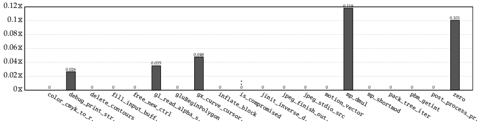
Figure 7.2: Normalized solution costs for two pattern sets: one without SIMD instructions (baseline), and one with such instruction (subject). GMI: 1.02\times , CI: [1.003, 1.03]\times . Functions whose bars are marked with two dots are those for which the subject does not find the optimal solution.
