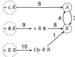
(b) Example of an LR graph based on the expression tree + \emptyset + c c and the grammar on the left-hand side. Dashed nodes represent subtrees of the expression tree and fully drawn nodes represent goals. Edges indicate rule applications, with the number of the applied rule appearing next to the edge.
