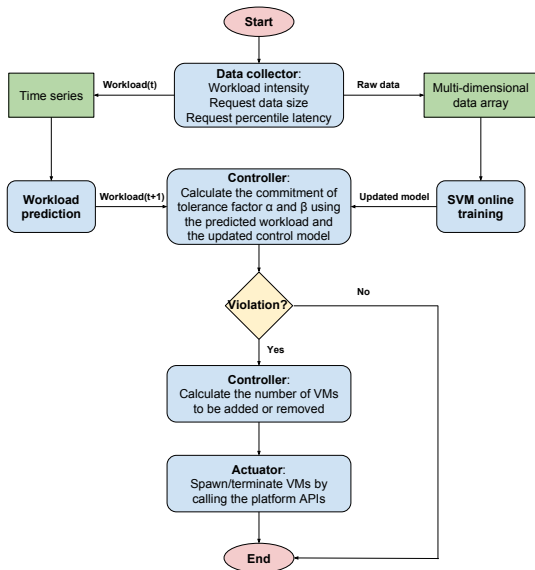
Fig. 6: Control flow of OnlineElastMan
