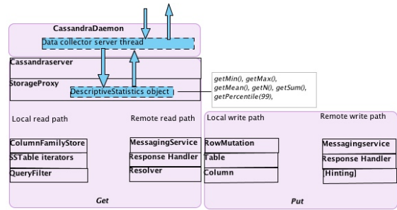
Fig. 8: Cassandra instrumentation to collect request latencies
