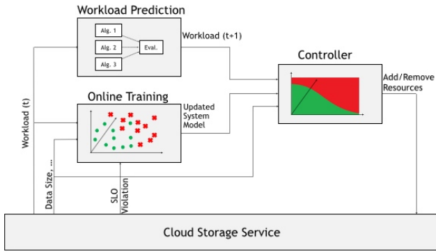
Fig. 1: OnlineElastMan Architecture
