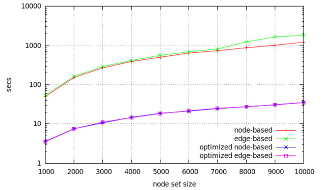
Figure 10: Performance improvement when using the affected subgraph discovery algorithm on structured network overlays with varying size and 20 outgoing flows per node.
