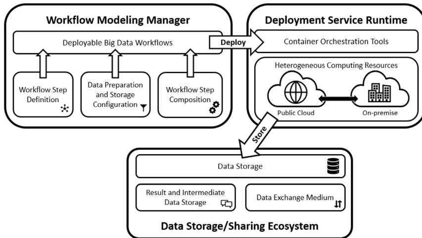
Fig. 1. Overview of the our workflow system.
