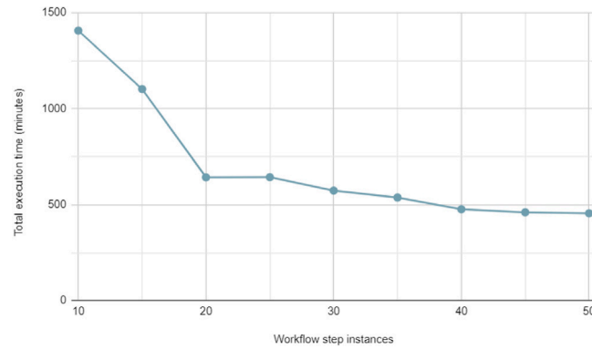
Fig. 5. Results of the horizontal scalability test.
