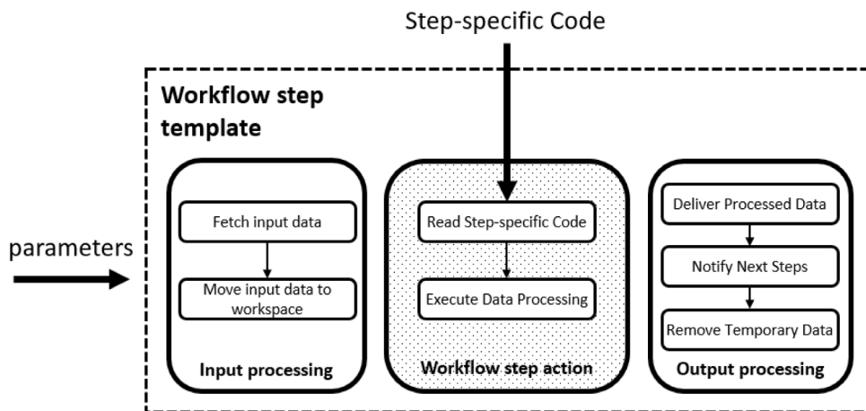
Fig. 3. Components of workflow step template.
