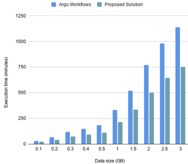
Fig. 7. Performance with increasing input size.
