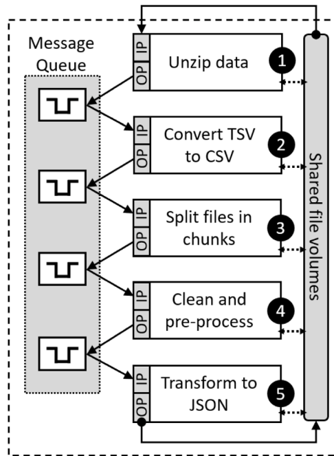
Fig. 4. Prototype Big Data workflow.
