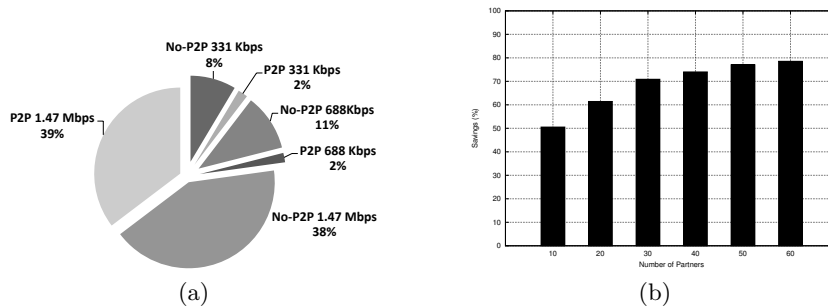
Fig. 4: (a) Breakdown of traffic quantities per bitrate using baseline, (b) Comparison of savings between different in-partners number.
